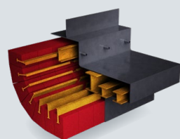
BULL NOSE PRESHAPED BLOCK SYSTEM for stressed areas
